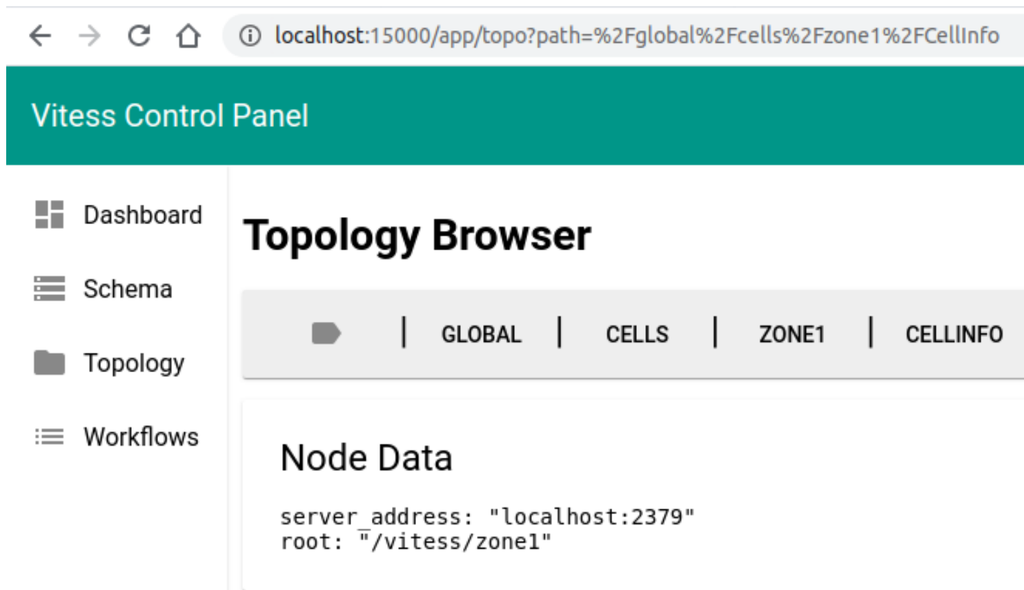
Figure 6: cell-in-topo
