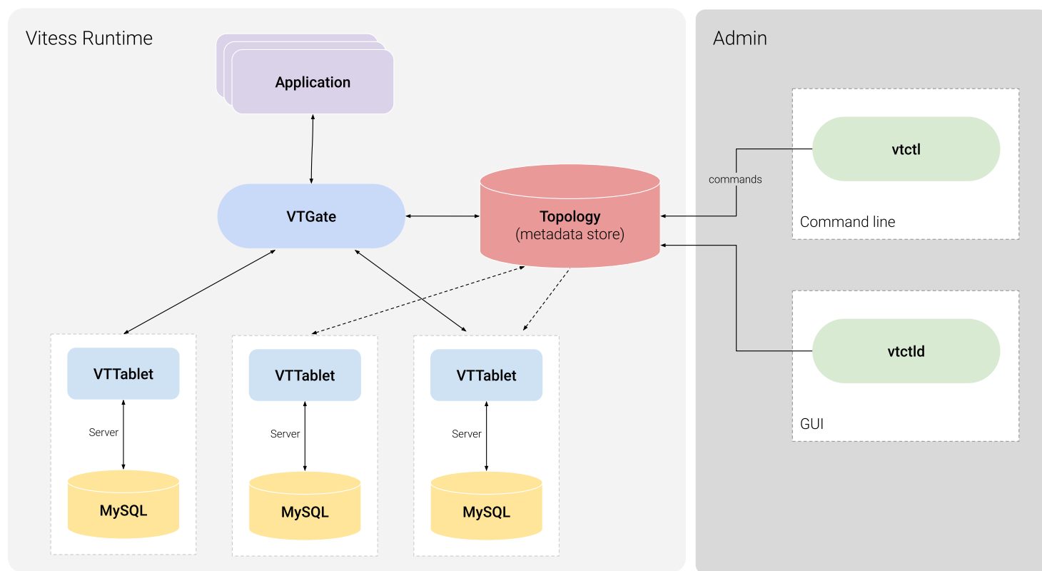
Figure 2: Architecture Diagram
